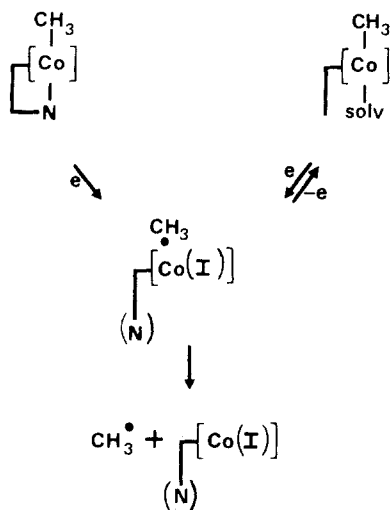
Scheme III Electrochemical Reduction of Methylcobalamin and Methylcobinamide
